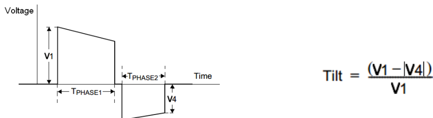
Figure 1. Biphasic PF 360J/100J Waveform
